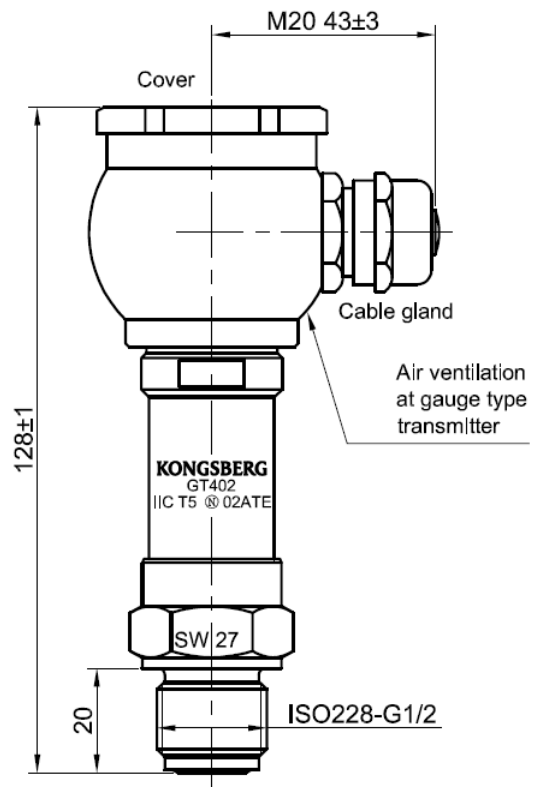
Figure 3: Dimensional sketch of GT402
