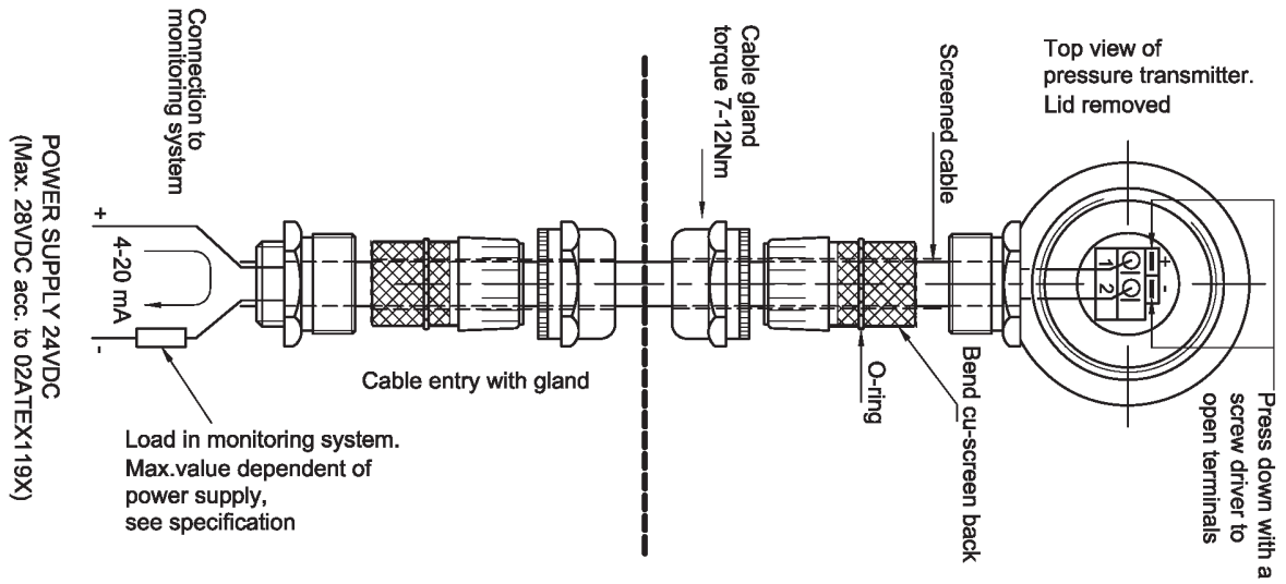
Figure 1: Electrical and mechanical installation of GT402
