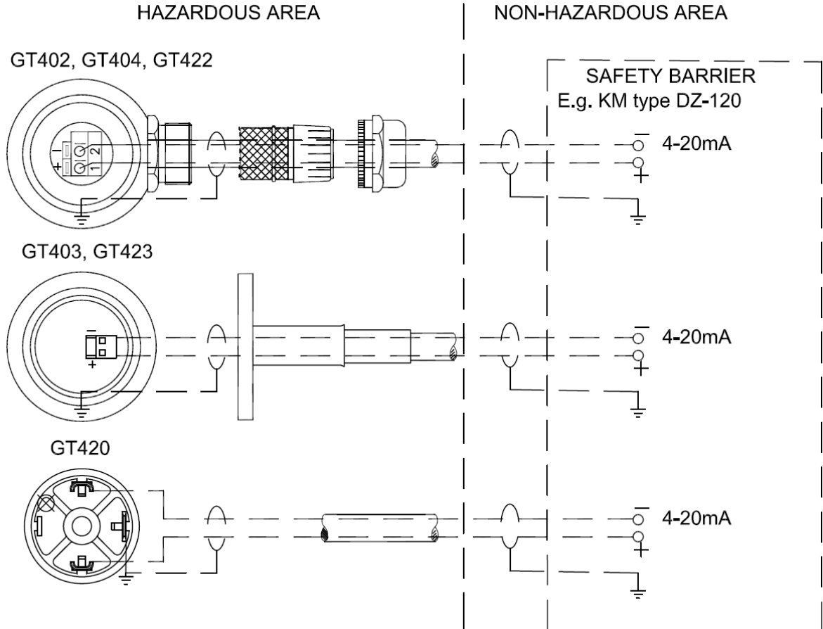
Figure 2: Connection diagram for Ex-area installations
